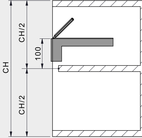
Tek Raf Uygulaması Single Shelf Application
