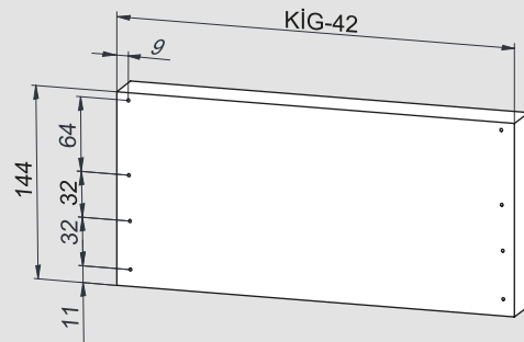
Arka Ahşap / Wooden Back Panel
