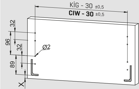
Ön Panel / Front Panel
