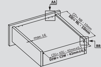
Drawer Dimensions
